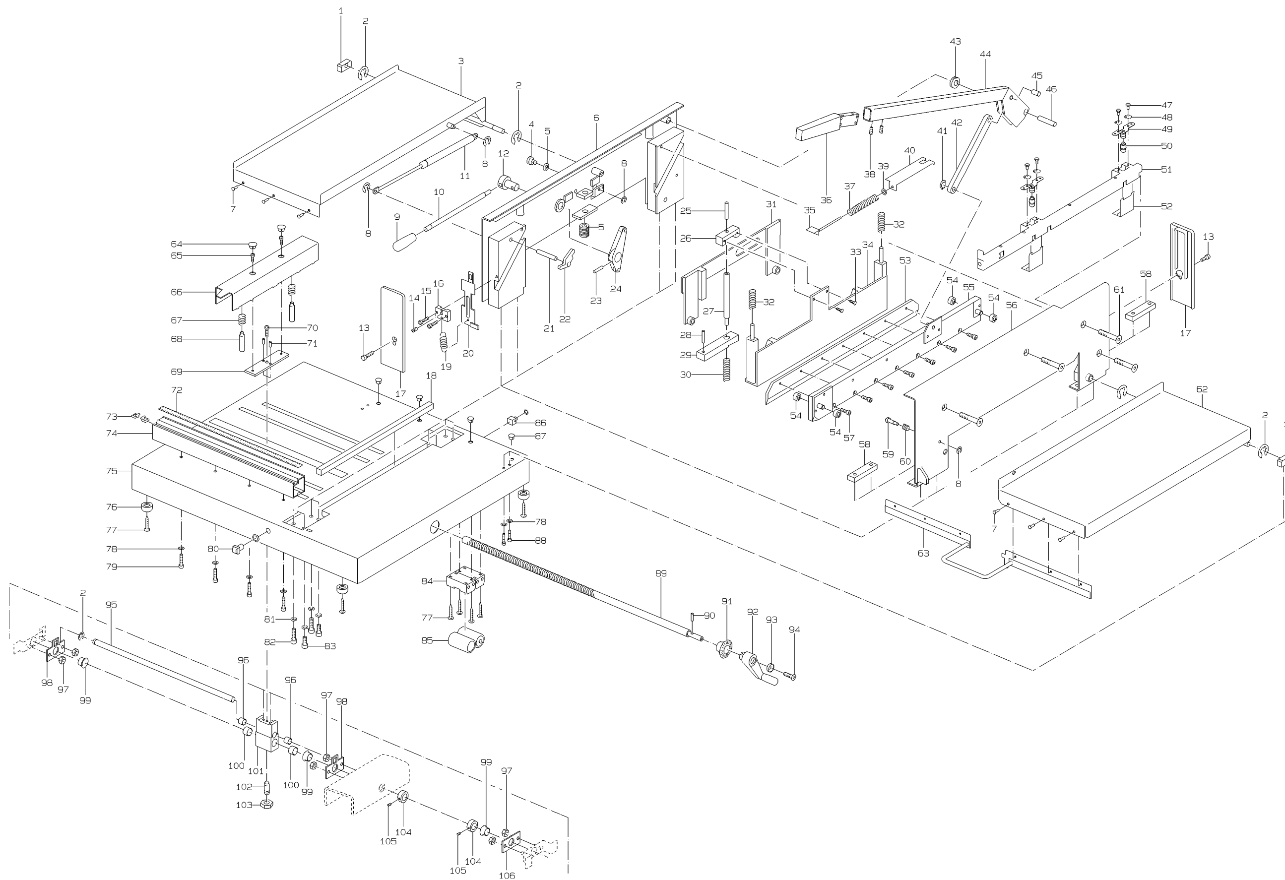
Abbildung 1 Stapelschneider 546 Illustration 1 Ream cutter 546 Illustration 1 Massicot 546
