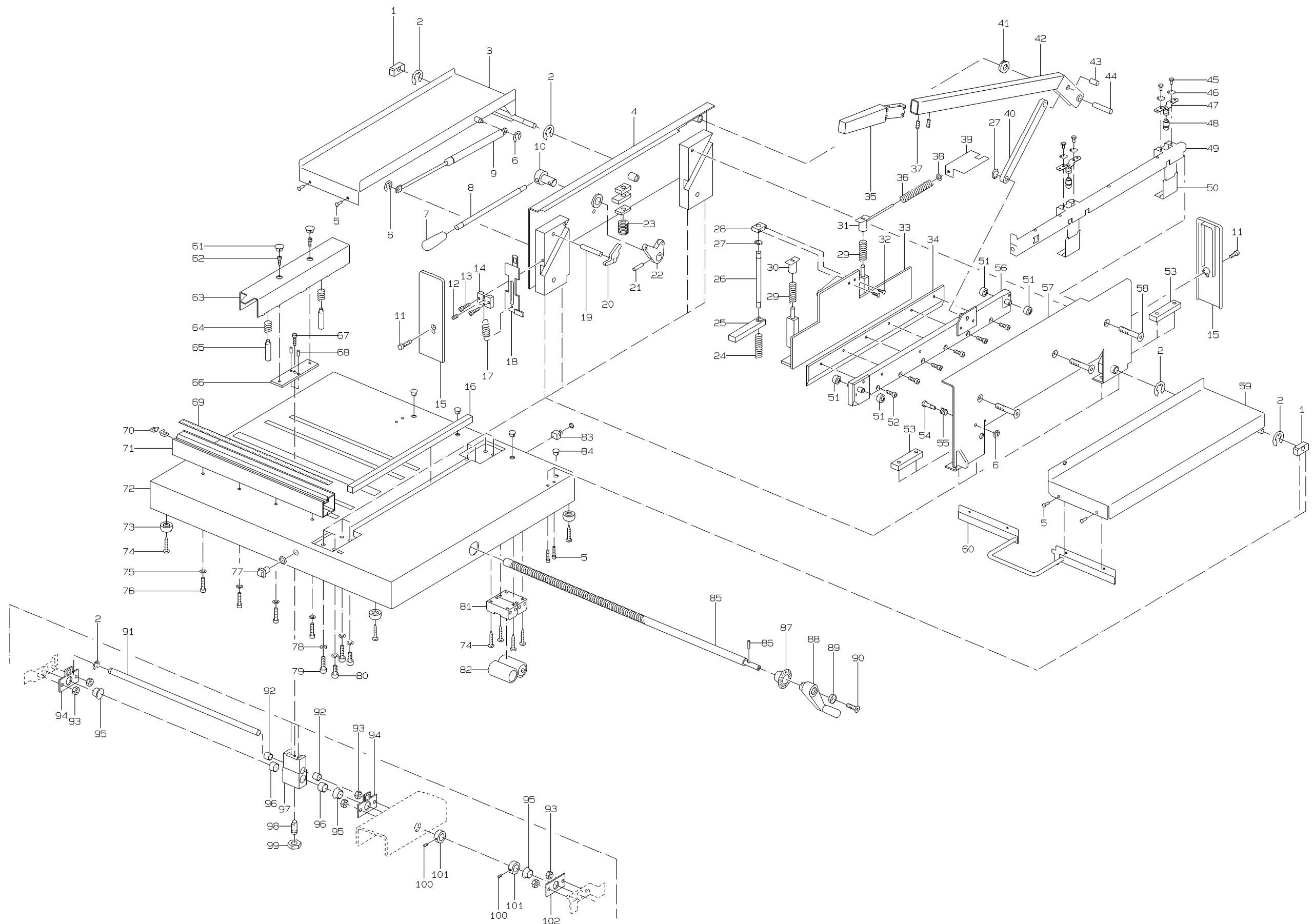
Abbildung 1 Stapelschneider 544 Illustration 1 Ream cutter 544 Illustration 1 Massicot 544
