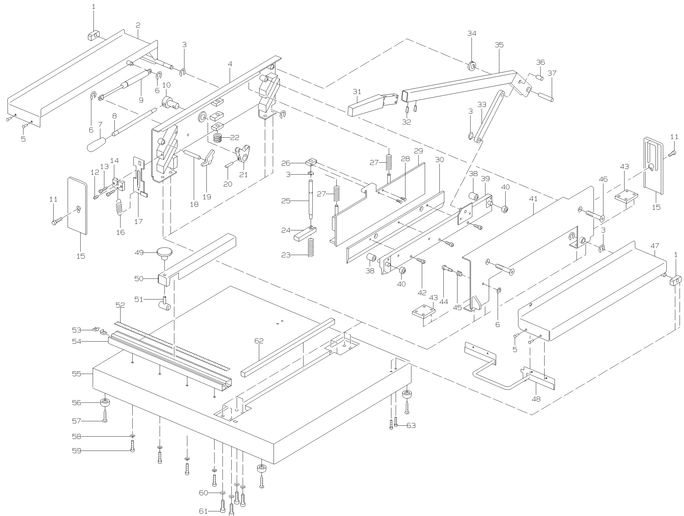
Abbildung 1 Stapelschneider 542 Illustration 1 Ream cutter 542 Illustration 1 Massicot 542
